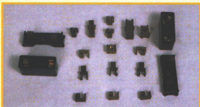
BRASS CONTACT BLOCKS FOR HRC FUSE CARRIERS
